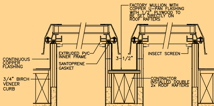
Factory Muller Curb
