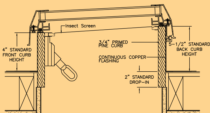
Flat Roof Drop-In Curb
