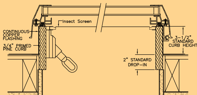
Pitched Roof Drop-In Curb
