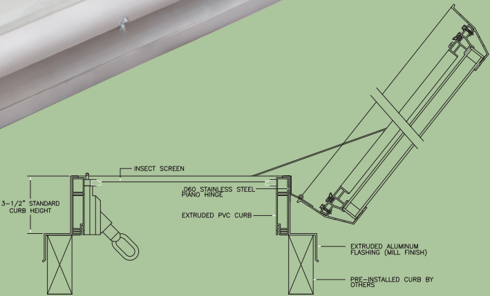
Vented Curb Mount
