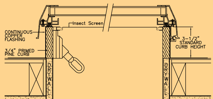
Cut Flush/Deck Mounted Curb
